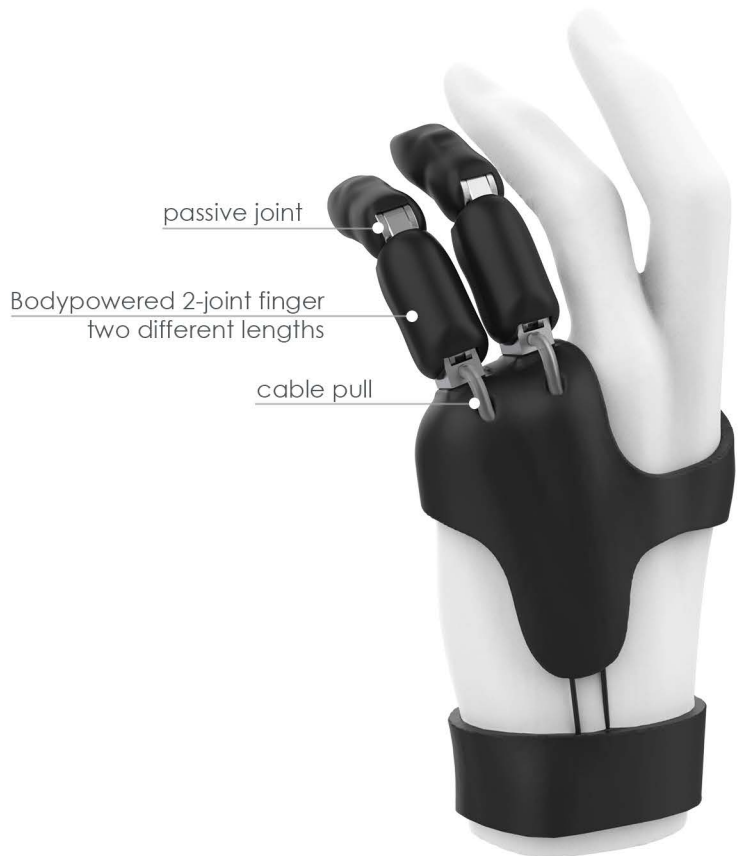
2-joint finger
